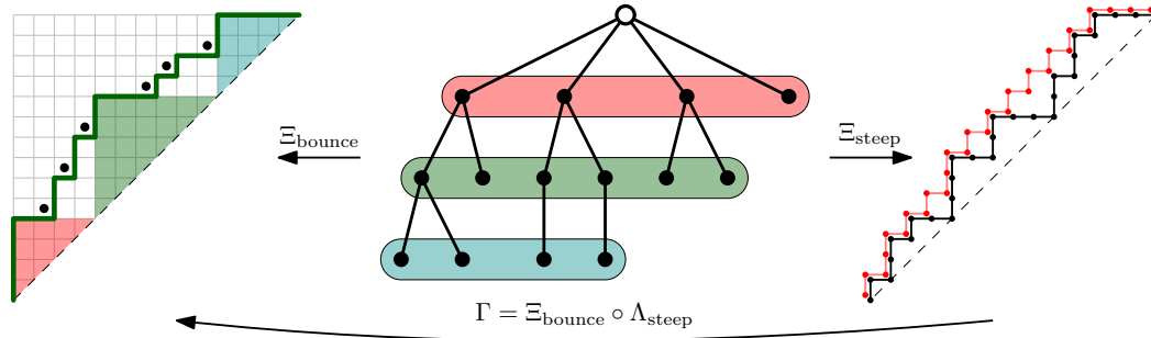
Figure 7: An illustration of the steep-bounce zeta map \Gamma .
