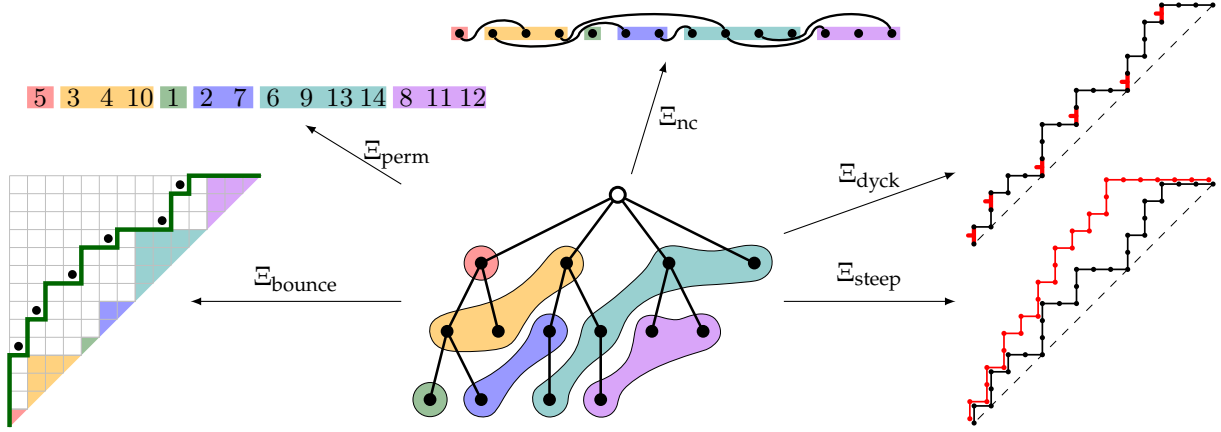
Figure 1: An overview of the bijections presented in this article.
