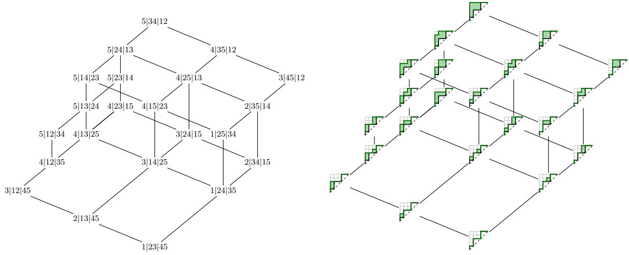
(a) The parabolic Tamari lattice \mathcal{T}_{(1,2,2)} .
