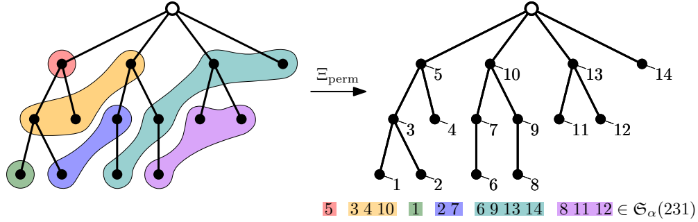
Figure 4: An illustration of the map \Xi_{\text{perm}} for \alpha = (1, 3, 1, 2, 4, 3) .
