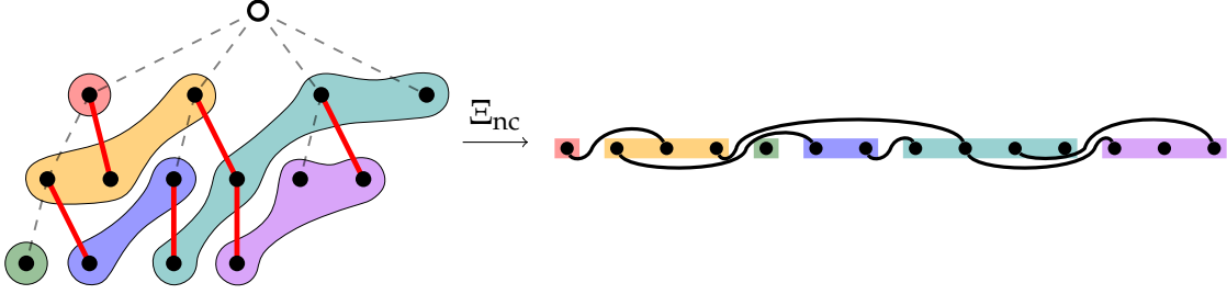
Figure 5: An illustration of the map \Xi_{nc} for \alpha = (1, 3, 1, 2, 4, 3) .
