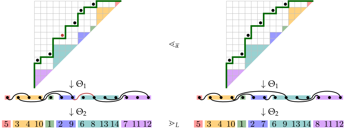
Figure 3: A cover relation in \mathcal{T}_{\alpha} and the corresponding cover relation in \mathcal{T}_{v_{\bar{\alpha}}} for \alpha = (1, 3, 1, 2, 4, 3) .
