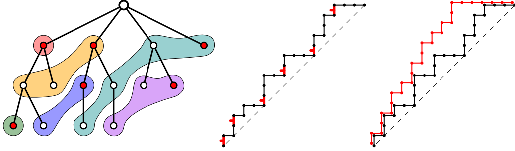
Figure 6: Illustrations of the maps \Xi_{\text{dyck}} and \Xi_{\text{steep}} for n = 14 and \alpha = (1, 3, 1, 2, 4, 3) .
