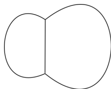
Figure 5: Metric graph of genus 2.
