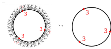
Figure 3: Weierstrass points on a genus 1 Berkovich curve, and retraction to a skeleton.
