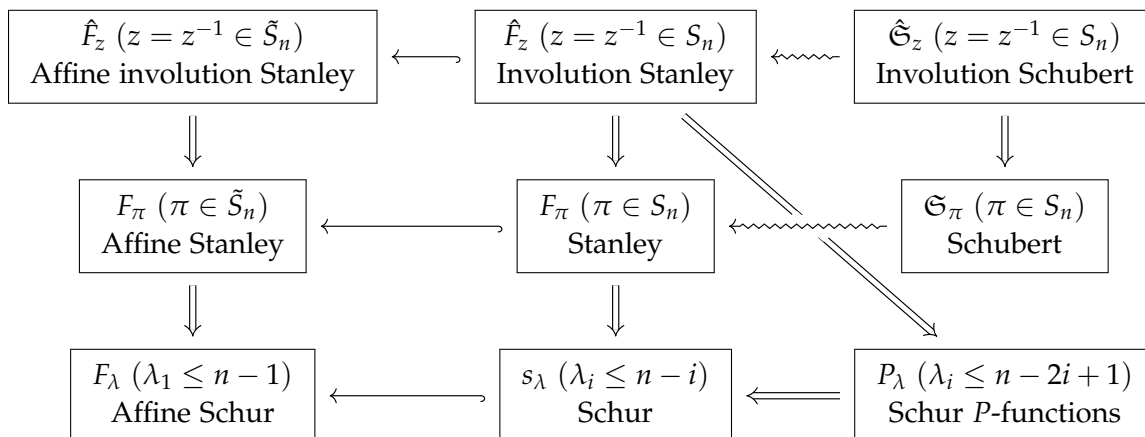
Figure 1: Families of polynomials and symmetric functions of interest. The relationships between each family are indicated as follows: \hookrightarrow means “is a special case of” while \rightsquigarrow means “has stable limit” while \Rightarrow means “expands positively into.”
