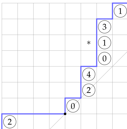
Figure 1: Example of an element in \text{PLSQ}^E(2, 6)^{*1} with reading word 241231.
